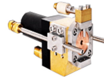
1.3 Plasma
